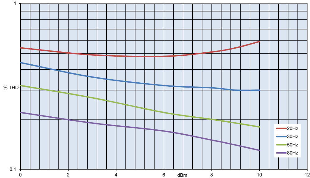
Distortion v input level @ fixed frequencies: secondary loaded with 9k7
