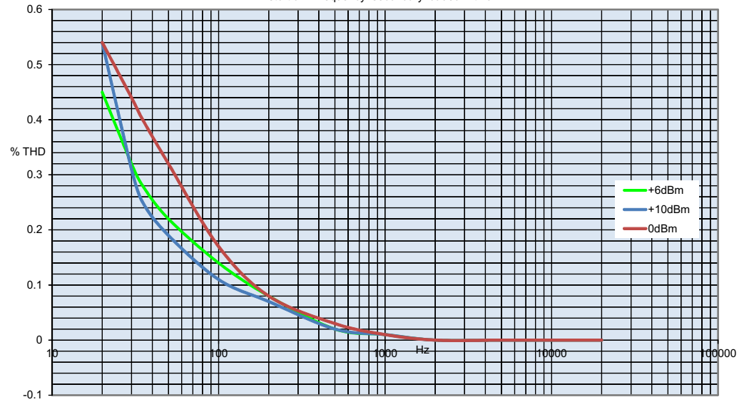
Distortion v frequency: secondary loaded with 9k7
