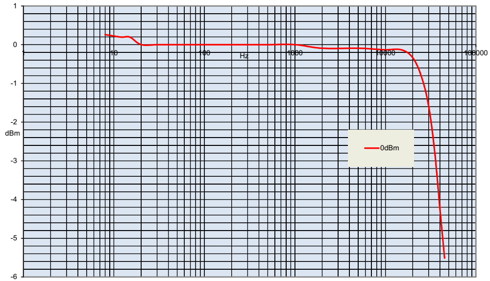
Frequency response: secondary loaded with 9k7
